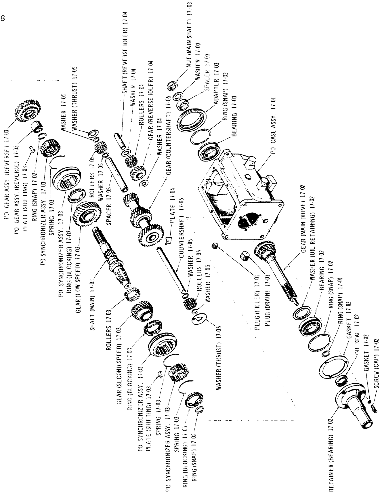
TRANSMISSION ASSEMBLY . . . T14A (CANE TYPE)
