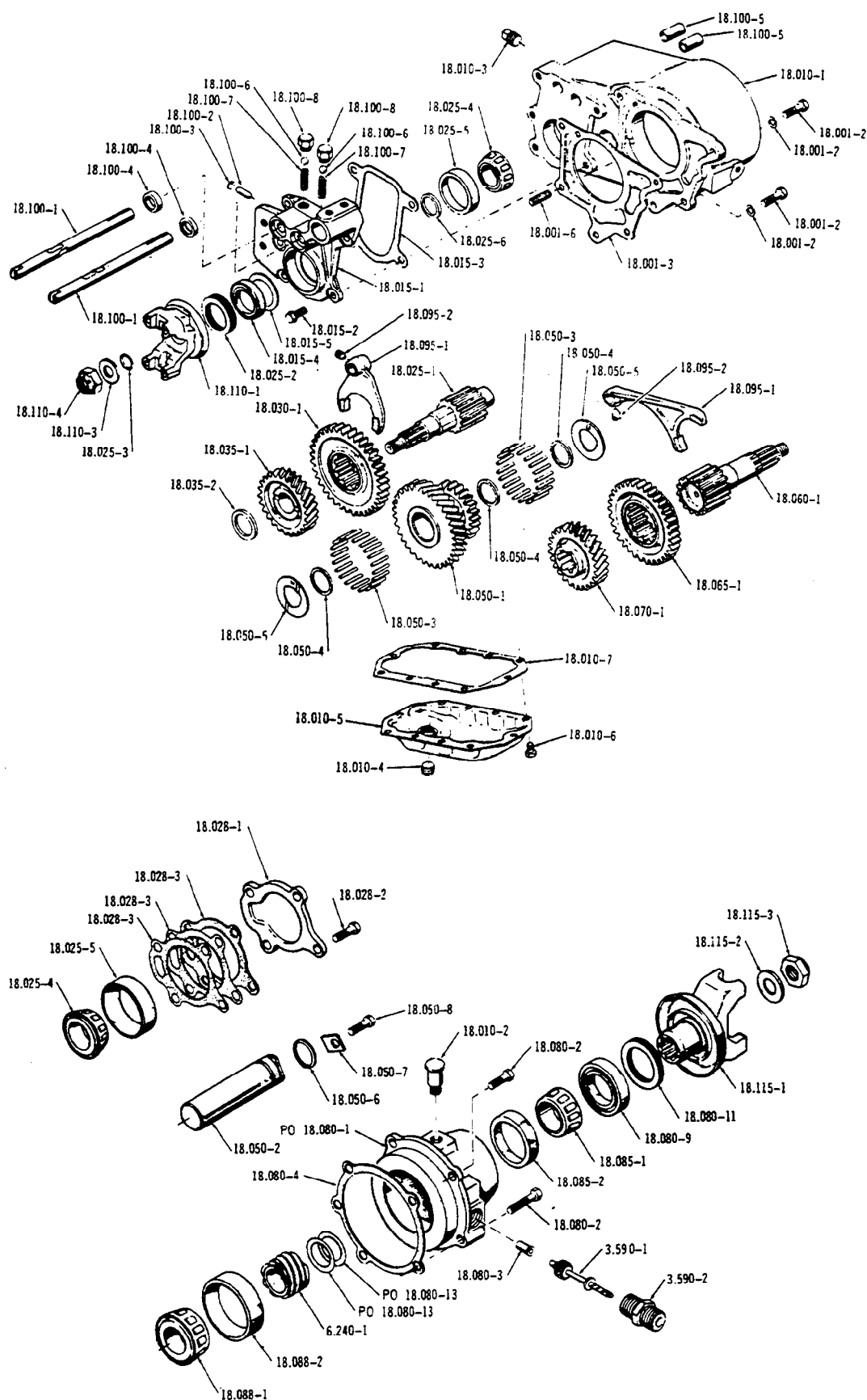
EXPLODED VIEW OF SILENT TYPE TRANSFER CASE
