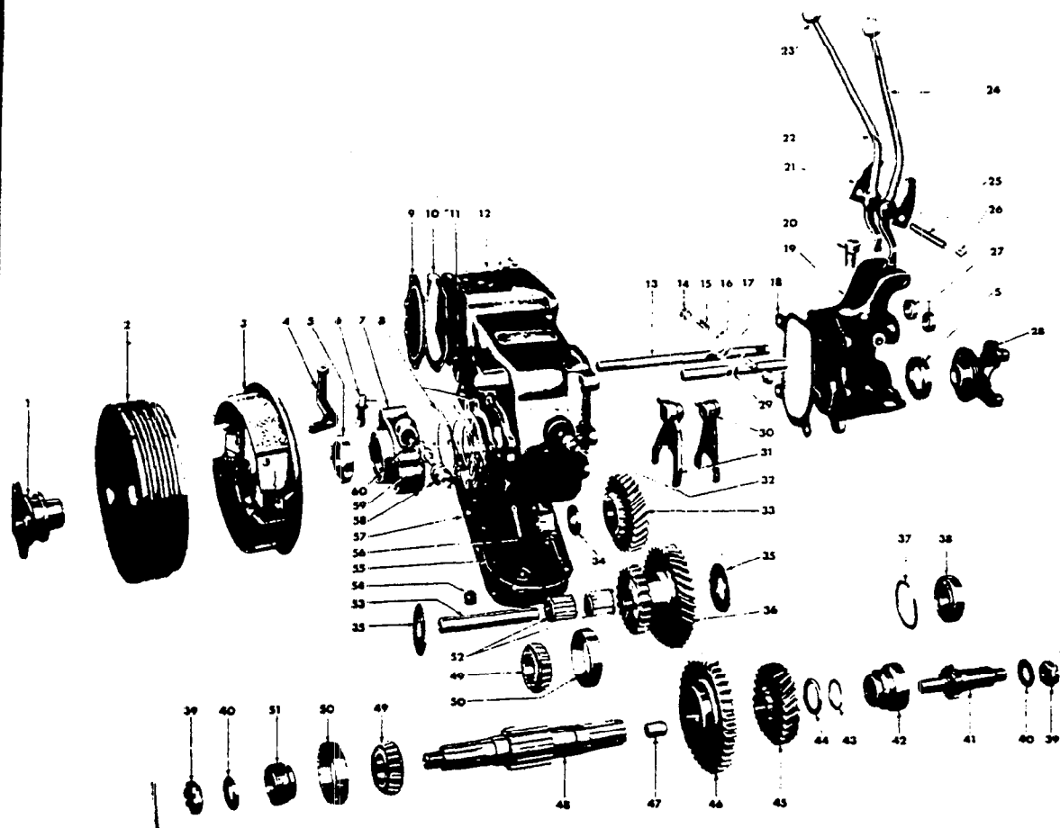
TRANSFER CASE EXPLODED VIEW (FOR MODELS CJ2A &amp; 3A)
