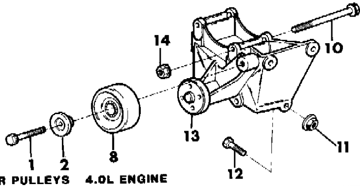
IDLER PULLEYS 4.0L ENGINE
