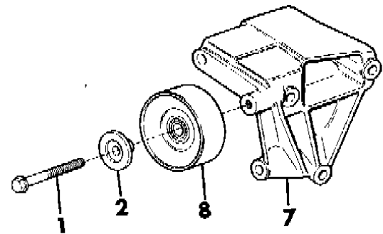
2.5L ENGINE
